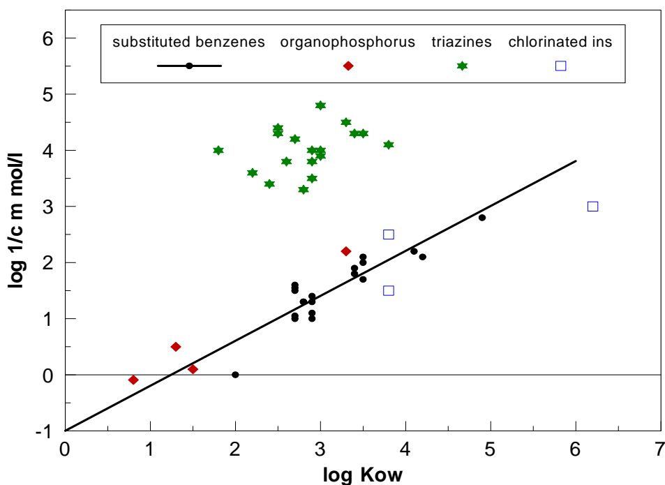
Figure 2 – Relationship between toxicity on algae (Log 1/EC 50 ) and Log K ow for chemicals with a specific (triazines) and a non-specific (all others) toxicological mode of action on algae (Vighi 2006).
