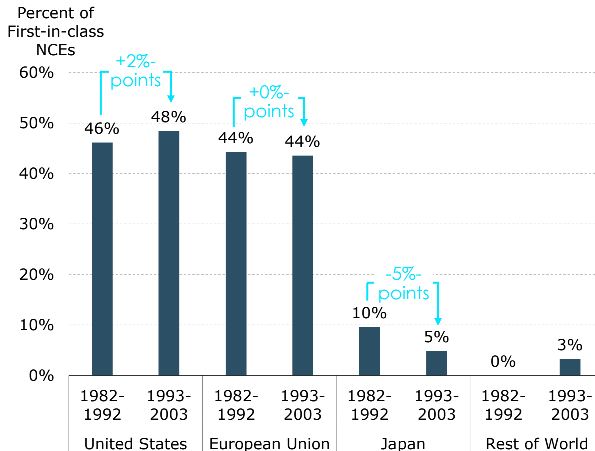
First-in-class New Chemical Entities (NCEs) discovered in the United States, Europe, Japan and the Rest of World, comparing the time period 1982-1992 to 1993-2003
