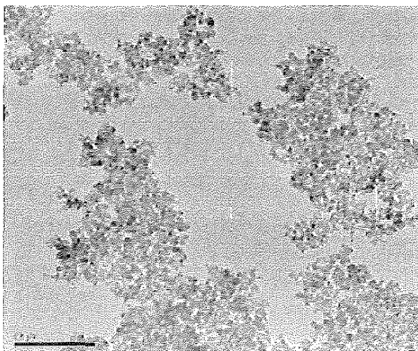
Fig. 5. TEM micrograph of dosing formulation used in safety studies: Unipure Black LC 902 in sodium carboxymethylcellulose (Sathish, 2012; Ramesh, 2012) Scale bar: 100 nm
